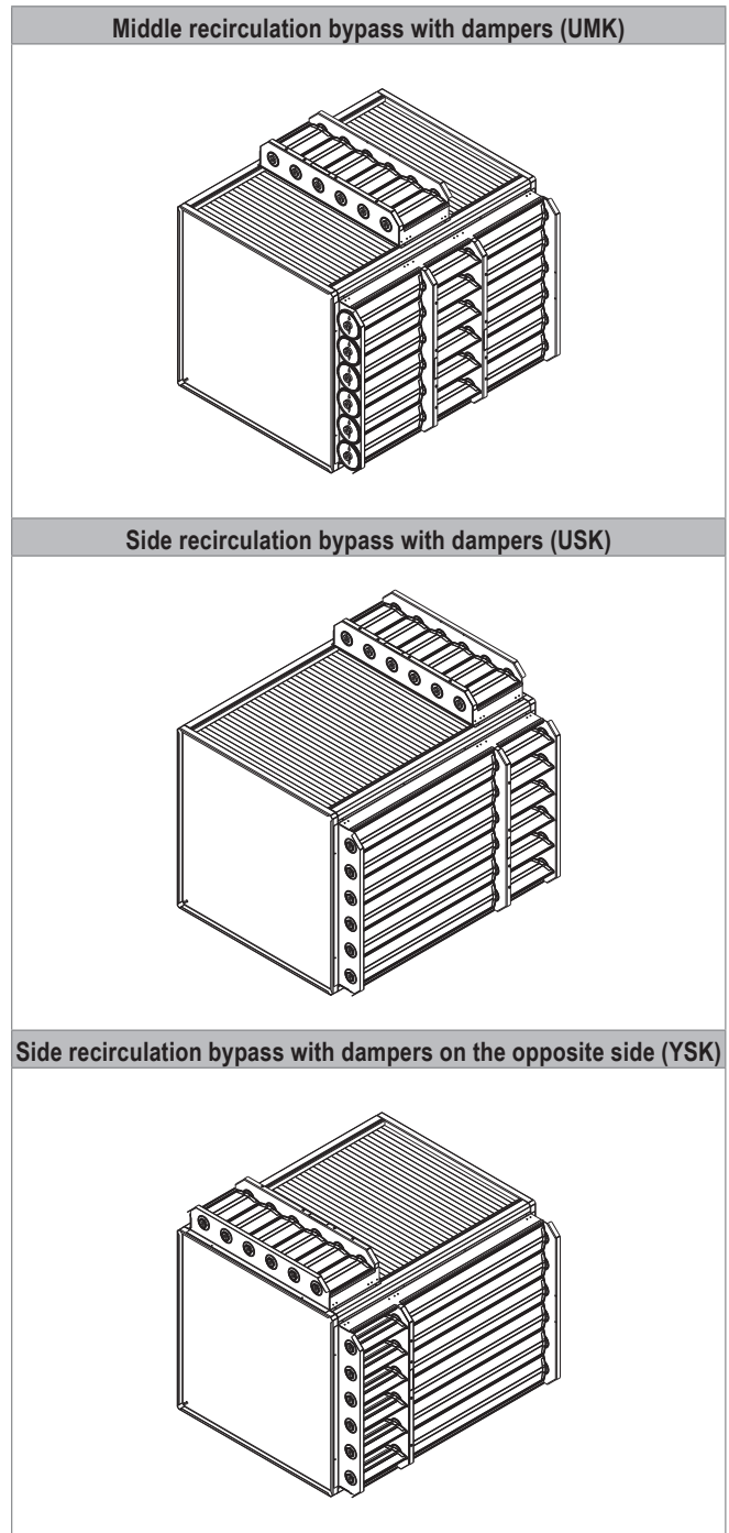
Fig. G10: Recirculation bypass variants
