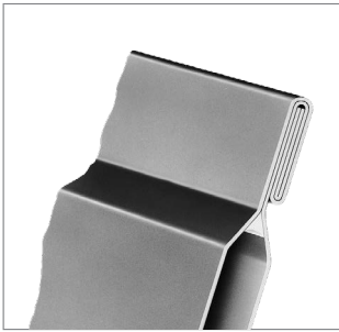
Fig. C4: Double fold connections give the exchanger package several-fold material thickness for the leading and trailing edges
