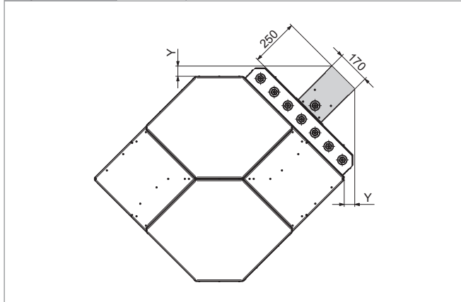
Fig. G7: Diagram showing dimensions of Gotthard combi block (in mm)
