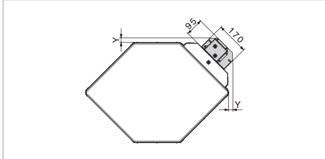
Fig. G6: Diagram showing dimensions of Gotthard (in mm)
