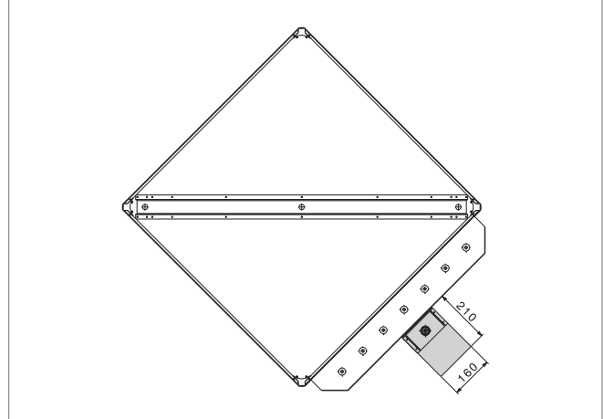
Fig. G9: Diagram showing dimensions of design F (in mm)
