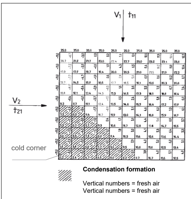
Figure 2: Temperature curve of a plate heat exchanger, calculated using the finite element method
