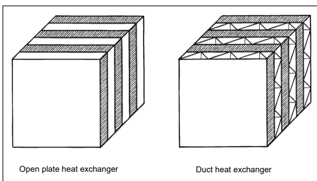
Figure 8: The internal structure of the plate heat exchanger is a decisive factor for the freezing behaviour.
