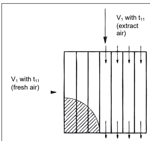
Figure 9: Air flow in partly frozen duct plate heat exchanger
